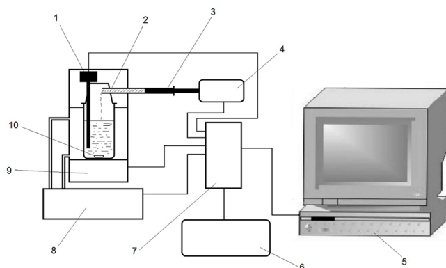
Figure 1. Schematic representation of the setup; 1: laser generator and photoelectronic convertor, 2: drug powder, 3: dispensing syringe, 4: syringe actuator, 5: display system, 6: power supply, 7: data processor and controller, 8: thermostate system, 9: magnetic stirrer, and 10: stir bar.
