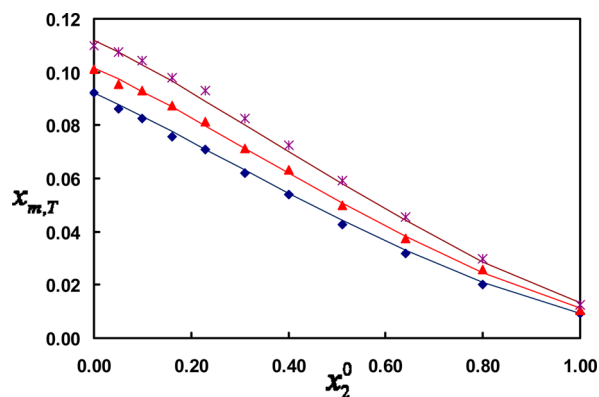
Figure 4. Comparison of predicted solubility data of TRIS in water + methanol mixtures (lines) at (298.2, 303.2, and 308) K with the corresponding experimental data (blue ♦, red ▲, or purple *).
