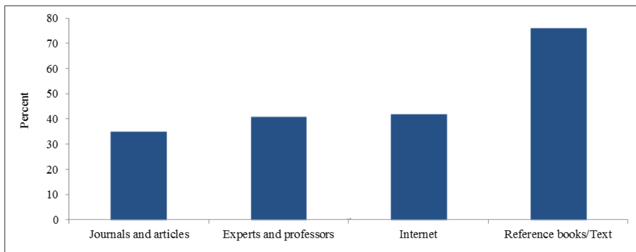
Figure 5. The used resources in evidence-based practice according to results of published papers
