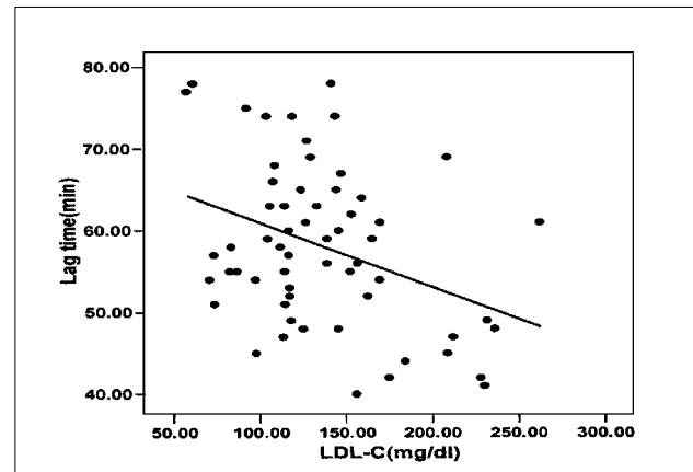
Figure 1 - Correlation between the serum low-density lipoprotein (LDL-C) and Lag time of LDL oxidation in the patient group ( r = -0.364 , p = 0.004 ).
