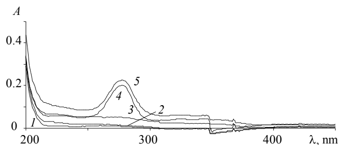
Fig. 2. Absorption spectra of \text{Tb}^{3+} (1), Hep (2), \text{Tb}^{3+} -Hep (3), \text{Tb}^{3+} -Dano (4), \text{Tb}^{3+} -Dano-Hep (5); [\text{Tb}^{3+}] = 4 \cdot 10^{-5} \text{ mol/l} , [\text{Dano}] = 2.5 \cdot 10^{-5} \text{ mol/l} , [\text{Hep}] = 1 \text{ } \mu\text{g/ml} , pH 7.2.
