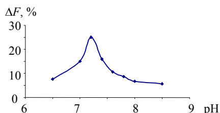
Fig. 3. Effect of pH; [\text{Tb}^{3+}] = 1 \cdot 10^{-5} \text{ mol/l} ; [\text{Dano}] = 2 \cdot 10^{-5} \text{ mol/l} ; [\text{Hep}] = 0.25 \text{ } \mu\text{g/ml} .
