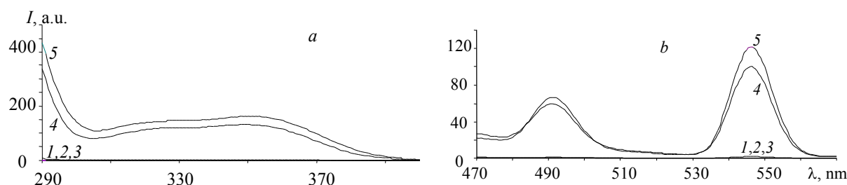
Fig. 1. Excitation (a) and emission (b) spectra of \text{Tb}^{3+} (1), Hep (2), \text{Tb}^{3+} -Hep (3), \text{Tb}^{3+} -Dano (4), and \text{Tb}^{3+} -Dano-Hep (5). Experimental conditions: [\text{Tb}^{3+}] = 4 \cdot 10^{-5} mol/l, [\text{Dano}] = 2.5 \cdot 10^{-5} mol/l, [\text{Hep}] = 0.25 \mu\text{g/ml} , pH 7.2, \lambda_{\text{ex}}/\lambda_{\text{em}} = 347 \text{ nm} / 545 \text{ nm} .
