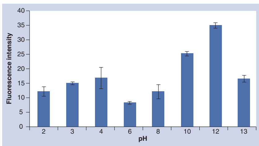
Figure 6. Effect of the sample solution pH on the extraction of carvedilol. Experimental conditions are the same as in FIGURE 5, and the optimized volume of disperser solvent is 0.5 ml.
