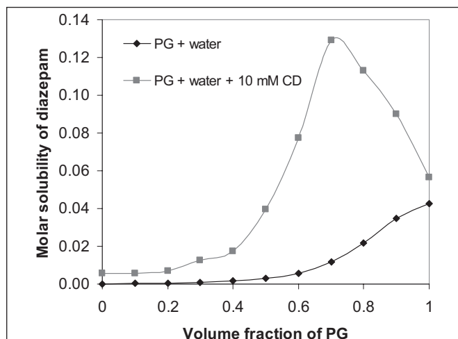
Figure 2 - Solubility profile of diazepam.
