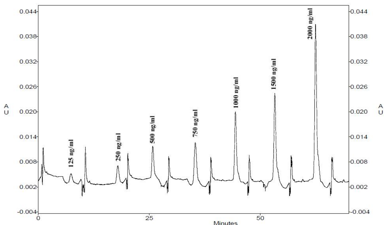
Figure 1. Chromatogram of serial concentrations of sirolimus
