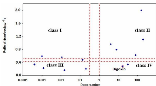
Fig 3: Classification of drugs based on dose number and rat P_{\text{eff}} values which were previously reported by authors [21,22]. Digoxin is added to this system as a class IV drug.
