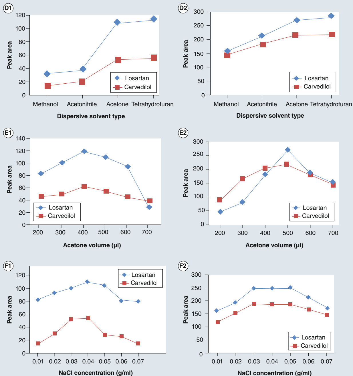
Figure 1. One factor at a time experimental design for the optimization of extraction procedure (cont.). Optimization of (D) dispersive type, (E) volume and (F) salt concentration in (1) urine and (2) plasma samples.
