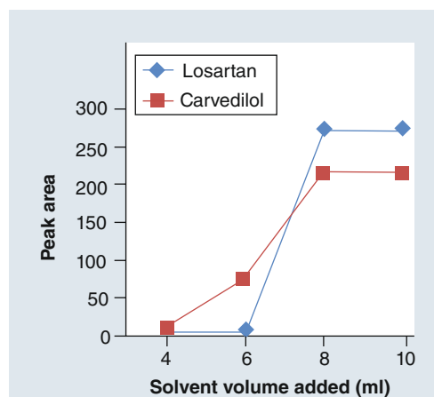
Figure 2. The effect of dilution of plasma samples on extraction.
