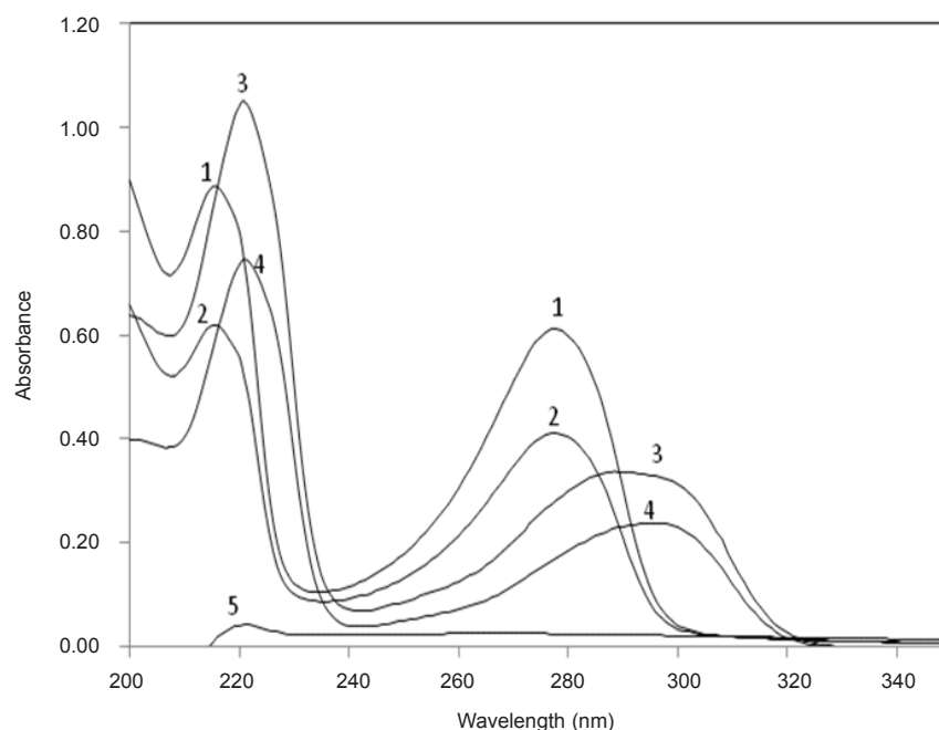
Figure 3. Absorption spectra of DFP in different systems (background correction was done by using a reference solution): DFP (1, 2); \text{Tb}^{3+} -DFP (3, 4) and \text{Tb}^{3+} (5). Conditions: [\text{Tb}^{3+}] = 1.0 \times 10^{-4} \text{ M} , [\text{DFP}] = 2.87 \times 10^{-5} \text{ M} (1, 3), 1.44 \times 10^{-5} \text{ M} (2, 4)
