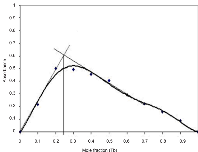
Figure 7. Determination of the stoichiometry of the terbium (III), conditions: DFP complex using Job's method; [DFP] and [\text{Tb}^{3+}] = 3.0 \times 10^{-4} M, pH=7.5.
