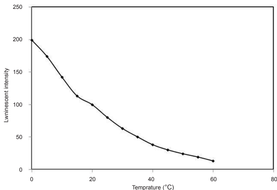
Figure 8. Effect of temperature, conditions: [\text{Tb}^{3+}] = 3 \times 10^{-4} \text{ M} , [\text{DFP}] = 7.2 \times 10^{-6} \text{ M} , \text{pH} = 7.5 .
