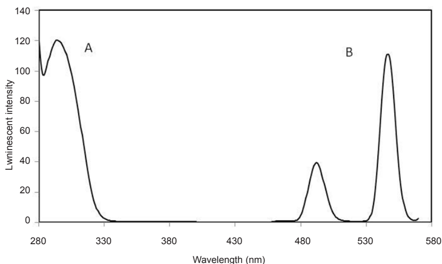
Figure 2. Luminescence excitation (A) and emission (B) spectra of: \text{Tb}^{3+} -DFP complex. Experimental conditions: [\text{Tb}^{3+}] = 10^{-5} M; [\text{DFP}] = 7.2 \times 10^{-6} M; pH = 7.5; \lambda_{\text{ex}}/\lambda_{\text{em}} = 295 \text{ nm}/545 \text{ nm} .
